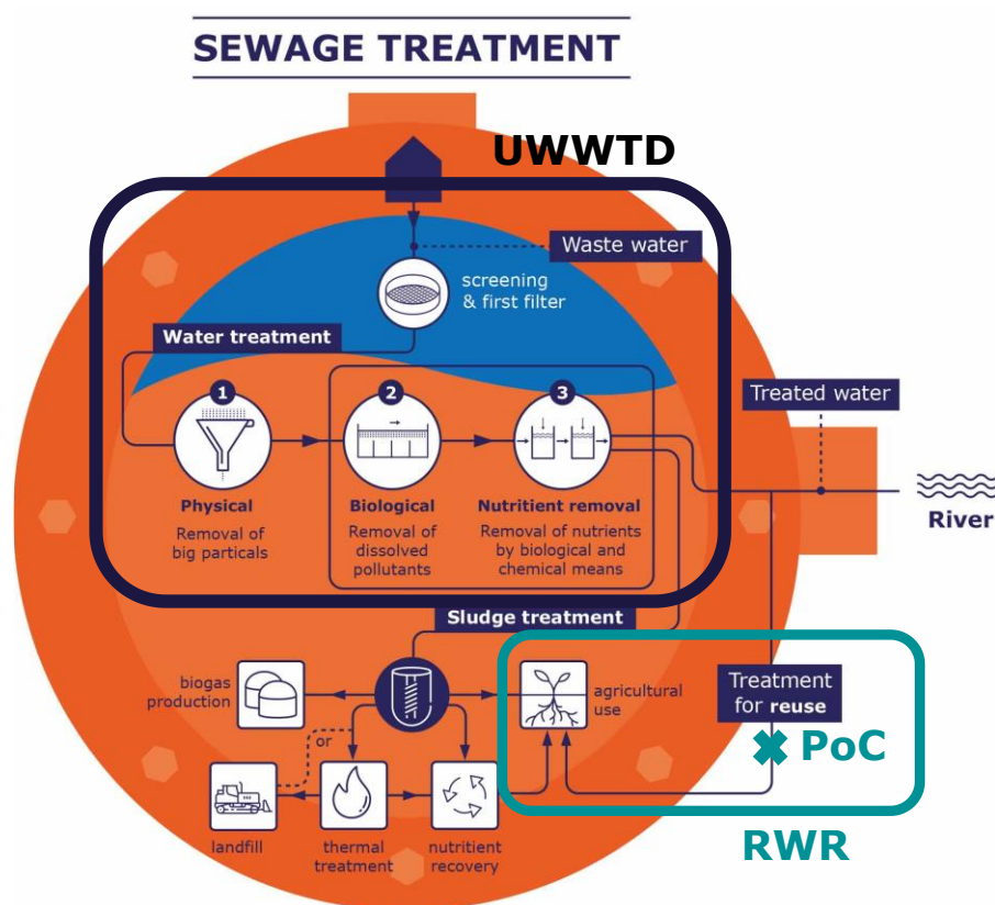
Figure 1: Scope of the Urban Waste Water Treatment Directive (UWWTD), the proposed Regulation on Water Reuse (RWR) and point of compliance of the regulation (PoC)
